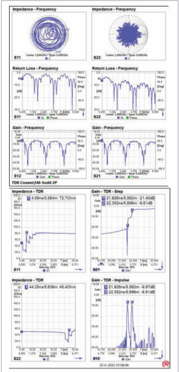
6. Shown are the measurements of the network with uneven signal paths. Note the two-step arrival, which is clearer with the impulse mode of the TDR transform.
