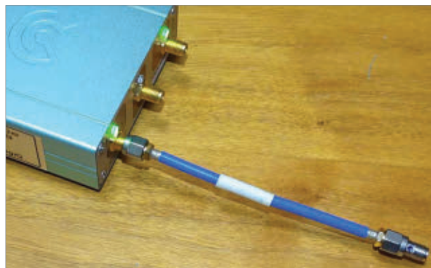
1. Here's the setup of a simple network measurement of a length of 50-Ω coax terminated with a short. Measurement results are provided in Figure 2 . Photo credits: MegiQ
