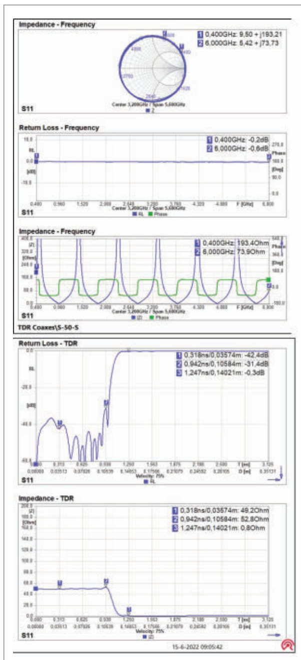
2. These graphs show the frequency and TDR measurement of the simple coax-cable network of Figure 1 .
